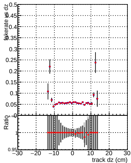
—•— DQM_V0001_R0000000001_Global_mkFitbase_RECO —•— DQM_V0001_R0000000001_Global_CMSSW_X_Y_Z_RECO
