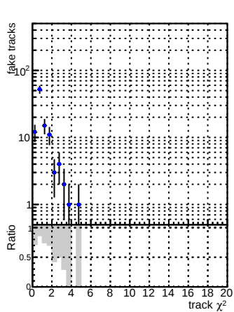
Legend: - Blue circle: DQM_V0001_R0000000001_Global_mkFitbase_RECO - Red circle: DQM_V0001_R0000000001_Global_CMSSW_X_Y_Z_RECO
