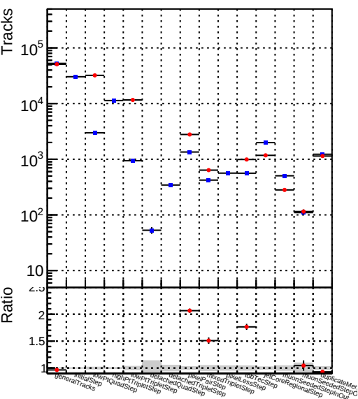
DQM_V0001_R000000001_Global_mkFitbase_RECO
