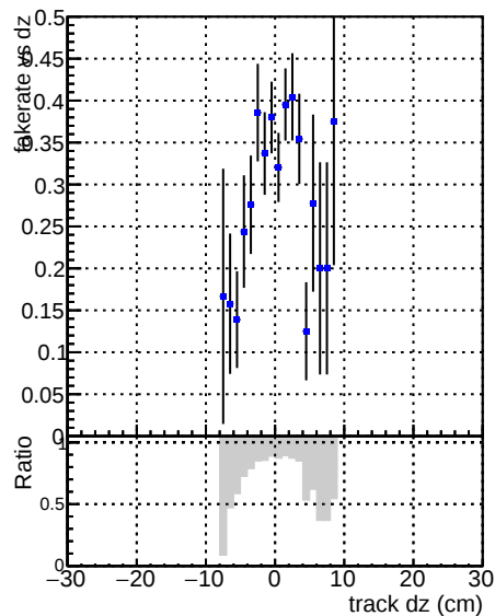
Fake rate vs dz Legend: Blue dots: DQM V0001_R000000001 Global mkFitbase RECO Red dots: DQM V0001_R000000001 Global mkSSW X Y Z RECO
