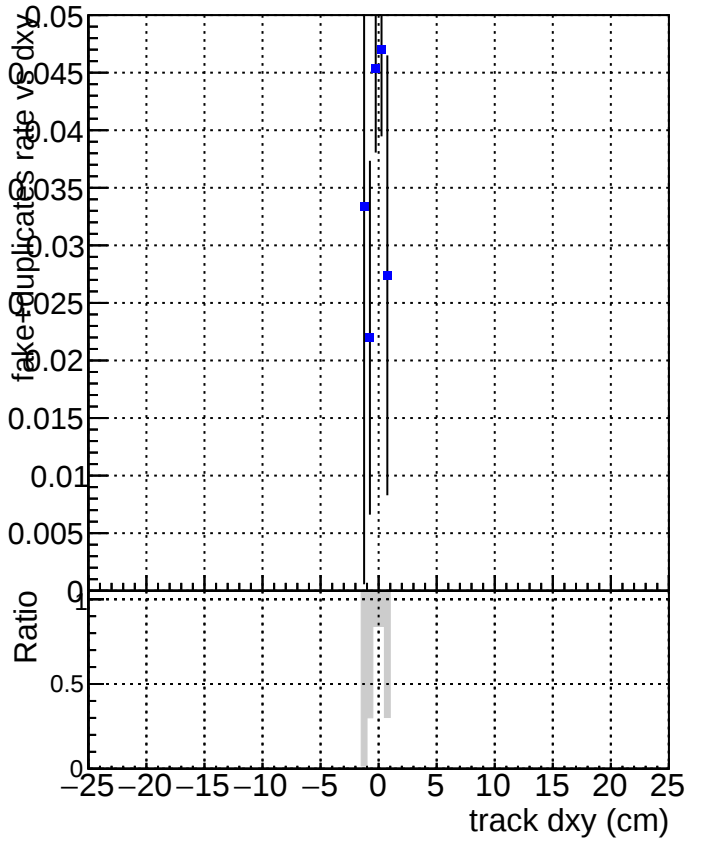
DQM_V0001_R000000001_Global_mkFitbase_RECO DQM_V0001_R000000001_Global_CMSSW_X_Y_Z_RECO
