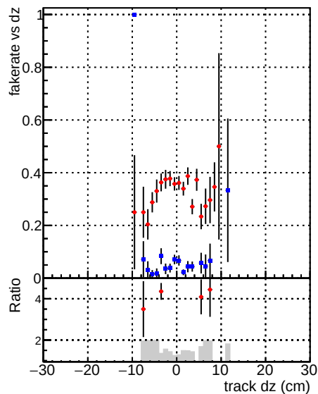
Fake rate vs dz —●— DQM V0001_R0000000001 Global —●— DQM V0001_R0000000001 Global —●— mkFitbase RECO —●— CMSSW X Y Z RECO
