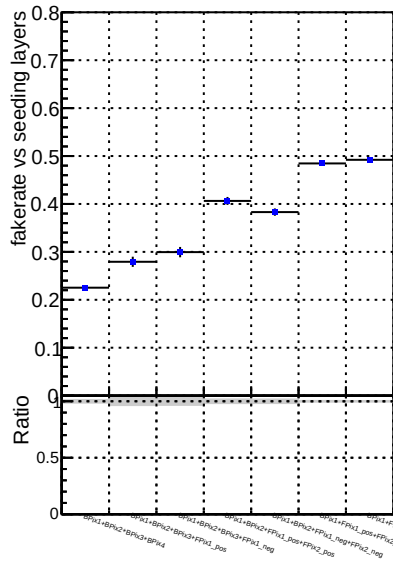
Fake rate vs. —•— DQM V0001_R000000001 Global mkFitbase RECO —•— DQM V0001_R000000001 Global CMSSW X Y Z RECO
