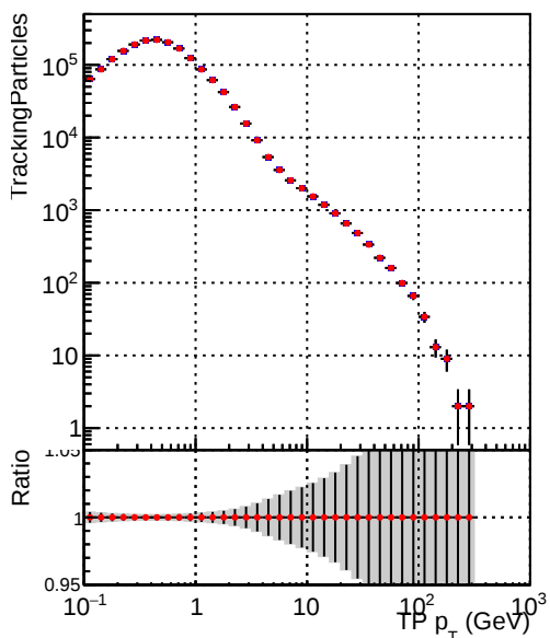
—•— DQM_V0001_R000000001_Global_mkFitbase_RECO - - - DQM_V0001_R000000001_Global_CMSSW_X_Y_Z_RECO
