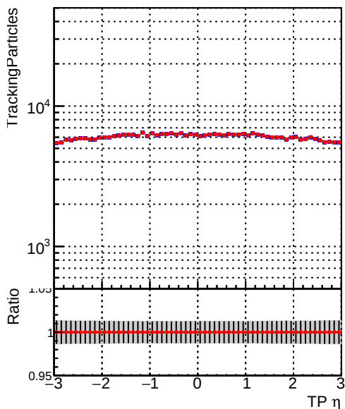
—•— DQM_V0001_R000000001_Global_mkFitbase_RECO - - - DQM_V0001_R000000001_Global_CMSSW_X_Y_Z_RECO
