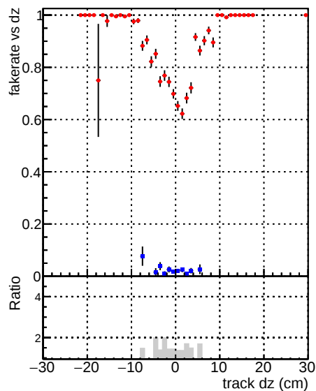
Fake rate vs dz DQM_V0001_R0000000001 Global mkFitbase RECO Global DQM_V0001_R0000000001 Global CMSSW_X_Y_Z RECO Global
