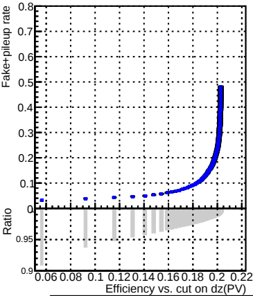
DQM_V0001_R000000001_Global_mkFitbase_RECO
