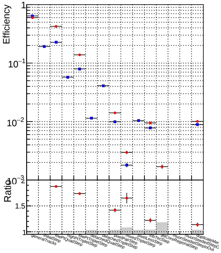
DQM_V0001_R000000001_Global_mkFitbase_RECO DQM_V0001_R000000001_Global_CMSSW_X_Y_Z_RECO
