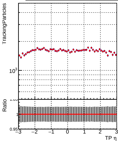
N of simulated tracks vs TP \eta Legend: - DQM_V0001_R000000001_Global_mkFitbase_RECO (Blue line with dots) - DQM_V0001_R000000001_Global_CMSSW_X_Y_Z_RECO (Red line with dots)
