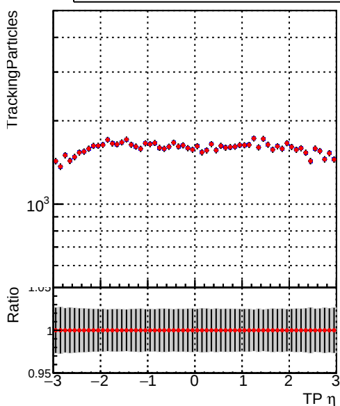
N of simulated tracks vs TP \eta Legend: - Blue dots: DQM_V0001_R000000001_Global_mkFitbase_RECO - Red dots: DQM_V0001_R000000001_Global_CMSSW_X_Y_Z_RECO
