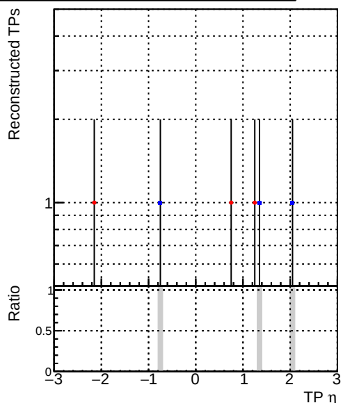
—•— DQM_V0001_R000000001_Global_mkFitbase_RECO —•— DQM_V0001_R000000001_Global_CMSSW_X_Y_Z_RECO
