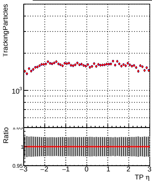
— DQM_V0001_R000000001_Global_mkFitbase_RECO — DQM_V0001_R000000001_Global_CMSSW_X_Y_Z_RECO
