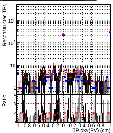
DQM_V0001_R000000001_Global_CMSSW_X_Y_Z_RECO
