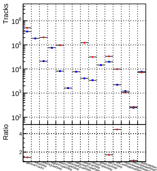
DQM_V0001_R000000001_Global_mkFitbase_RECO
