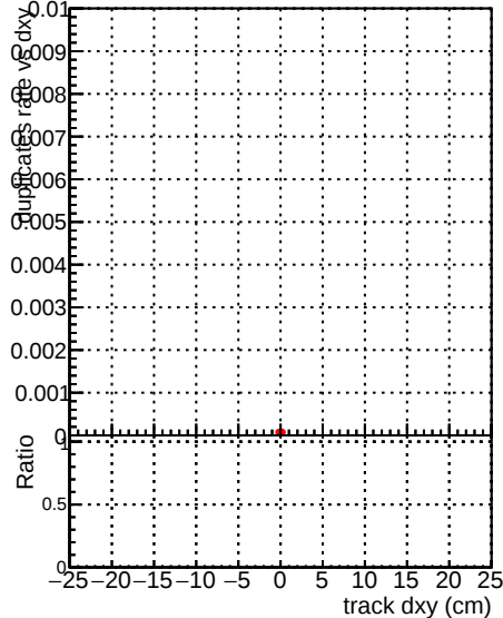
Global mkFitbase RECO DQM_V0001_R0000000001 Global CMSSW_X_Y_Z_RECO
