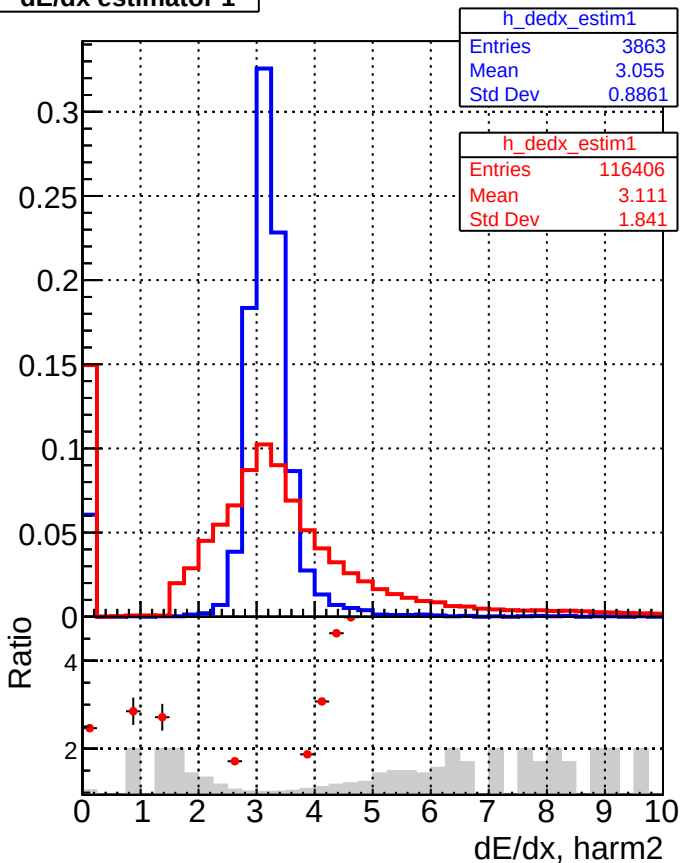
DQM_V0001_R000000001_Global_mkFitbase_RECO DQM_V0001_R000000001_Global_CMSSW_X_Y_Z_RECO
