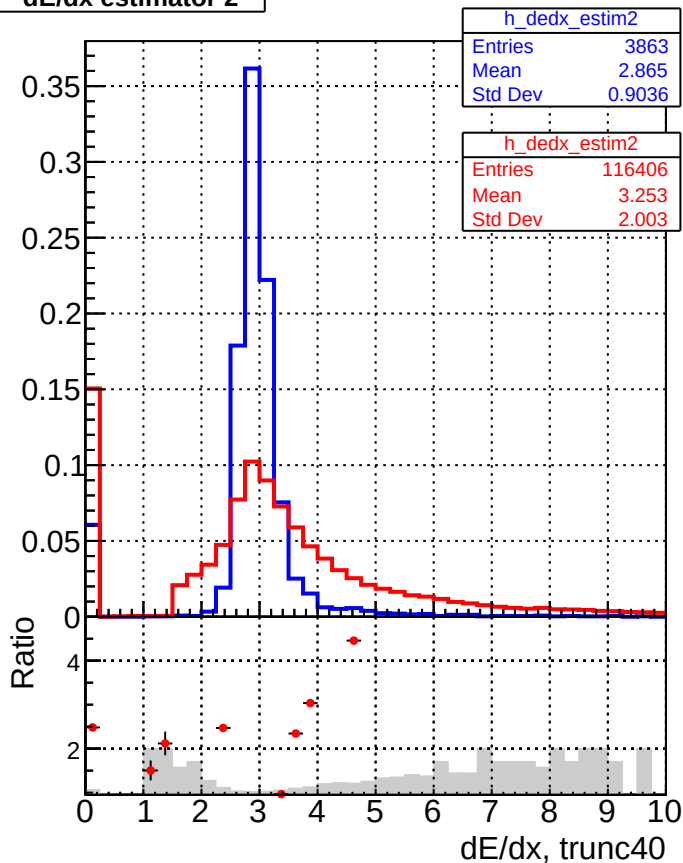
DQM_V0001_R000000001_Global_mkFitbase_RECO DQM_V0001_R000000001_Global_CMSSW_X_Y_Z_RECO
