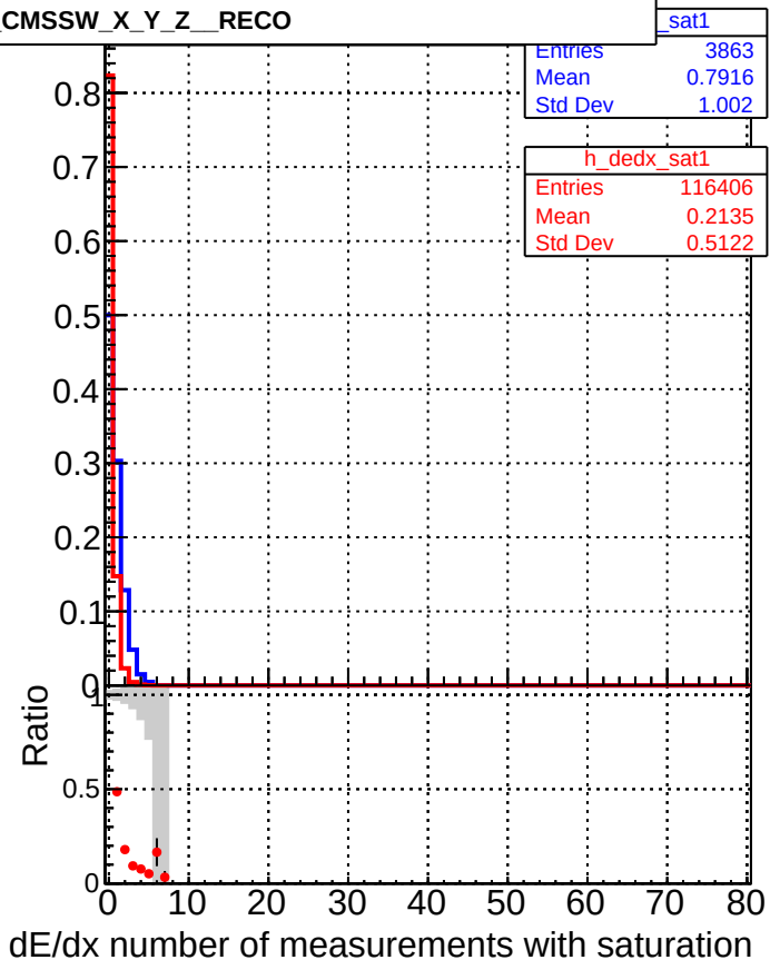
DQM_V0001_R000000001_Global_mkFitbase_RECO DQM_V0001_R000000001_Global_CMSSW_X_Y_Z_RECO
