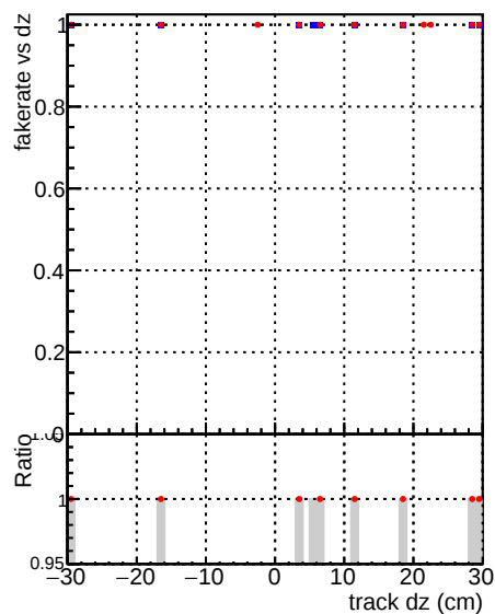
Fake rate vs dz DQM_V0001_R0000000001_Global_mkFitbase_RECO DQM_V0001_R0000000001_Global_mkSSW_X_Y_Z_RECO
