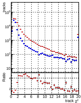
N of reco track vs. \chi^2 —●— DQM V0001 R000000001 Global mkFitbase RECO —●— DQM V0001 R000000001 Global CMSSW X Y Z RECO
