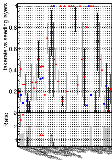
Fake rate vs. —◆— DQM_V0001_R000000001_Global_mkFitbase_RECO —◆— DQM_V0001_R000000001_Global_CMSSW_X_Y_Z_RECO
