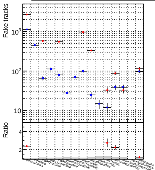
Number —●— DQM_V0001_R000000001_Global_CMSSW_X_Y_Z_RECO
