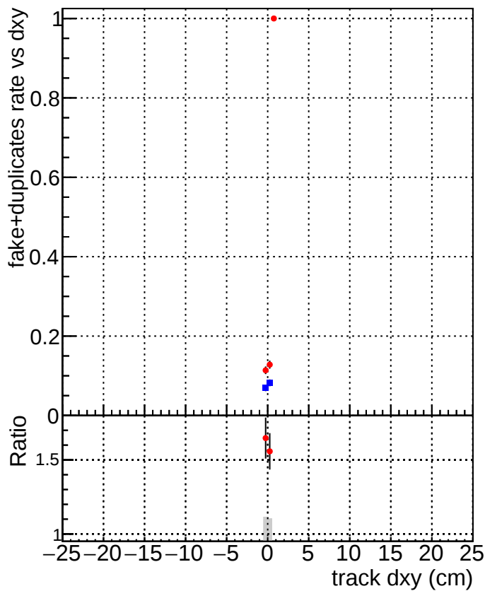
DQM_V0001_R000000001_Global_mkFitbase_RECO DQM_V0001_R000000001_Global_CMSSW_X_Y_Z_RECO
