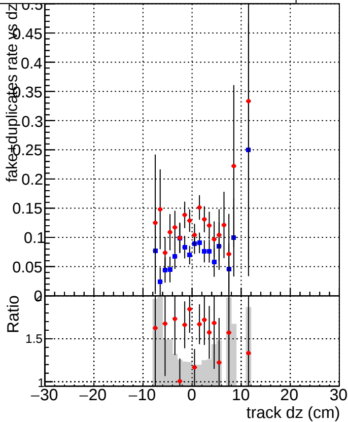
DQM_V0001_R000000001_Global_mkFitbase_RECO DQM_V0001_R000000001_Global_CMSSW_X_Y_Z_RECO
