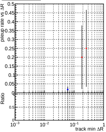
Legend: DQM_V0001_R000000001_Global_mkFitbase_RECO (blue dots), DQM_V0001_R000000001_Global_CMSSW_X_Y_Z_RECO (red dots)
