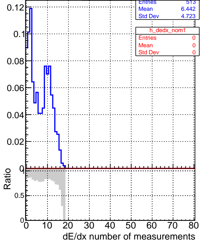
■ DQM_V0001_R000000001_Global_mkFitbase_RECO ● DQM_V0001_R000000001_Global_CMSSW_X_Y_Z_RECO
