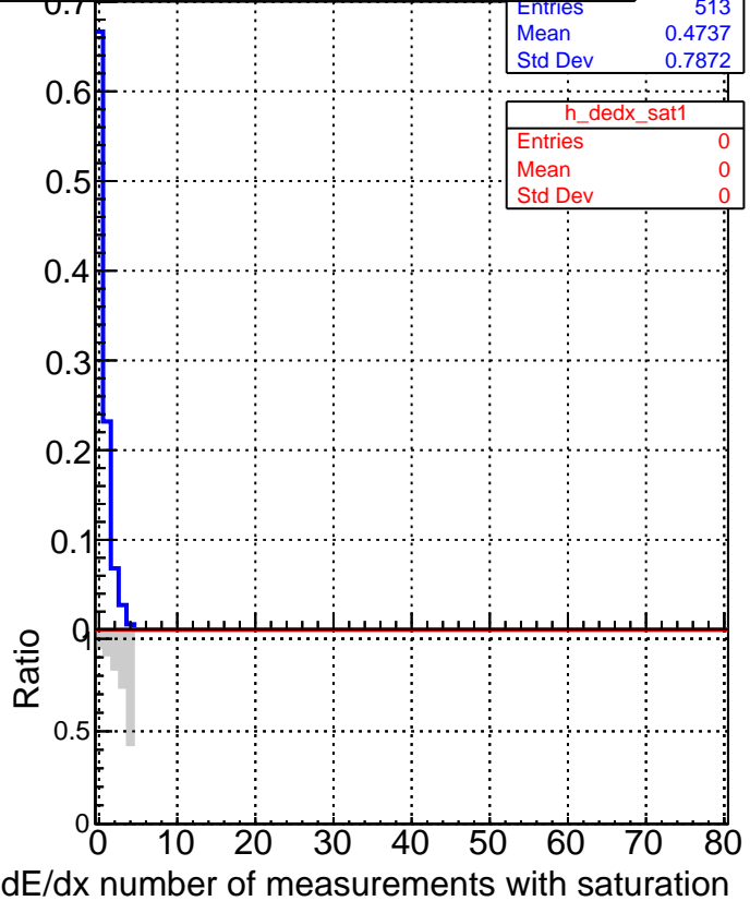
■ DQM_V0001_R000000001_Global_mkFitbase_RECO ● DQM_V0001_R000000001_Global_CMSSW_X_Y_Z_RECO
