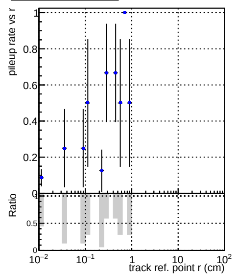
—●— DQM_V0001_R000000001_Global_mkFitbase_RECO —●— DQM_V0001_R000000001_Global_CMSSW_X_Y_Z_RECO
