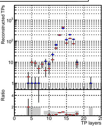
DQM_V0001_R000000001_Global_mkFitbase_RECO
