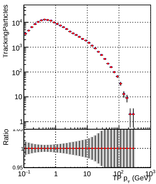
—•— DQM_V0001_R000000001_Global_mkFitbase_RECO —•— DQM_V0001_R000000001_Global_CMSSW_X_Y_Z_RECO
