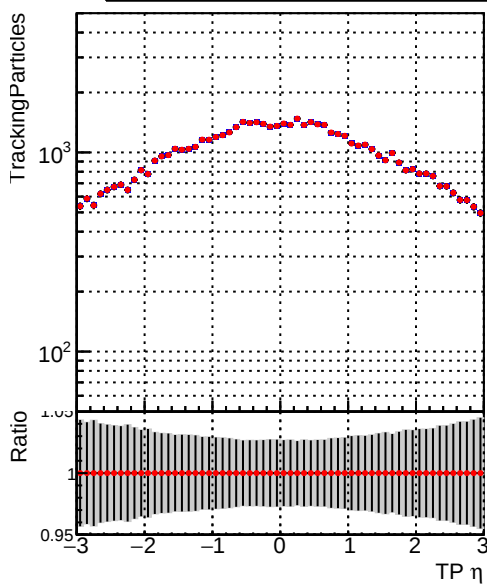
—•— DQM_V0001_R000000001_Global_mkFitbase_RECO —•— DQM_V0001_R000000001_Global_CMSSW_X_Y_Z_RECO
