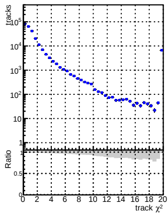
N of reco track vs. \chi^2 Blue dots: DQM V0001_R000000001 Global mkFitbase_RECO Red dots: DQM V0001_R000000001 Global CMSSW_X_Y_Z_RECO
