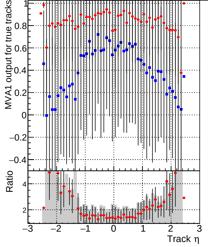
MVA1 of associated tracks (recoToSim) vs. track \eta Legend: Blue star: DQM_V0001_R000000001_Global_mkFitbase_RECO Red diamond: DQM_V0001_R000000001_Global_CMSSW_X_Y_Z_RECO
