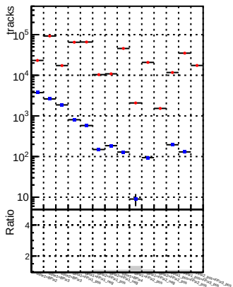
N of reco track vs. s DQM_V0001_R0000000001 Global mkFitbase RECO DQM_V0001_R0000000001 Global CMSSW_X_Y_Z RECO
