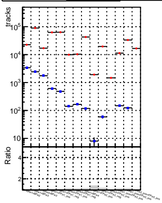
N of reco track vs. DQM V0001 R000000001 Global mkFitbase RECO DQM V0001 R000000001 Global CMSSW X_Y_Z_RECO
