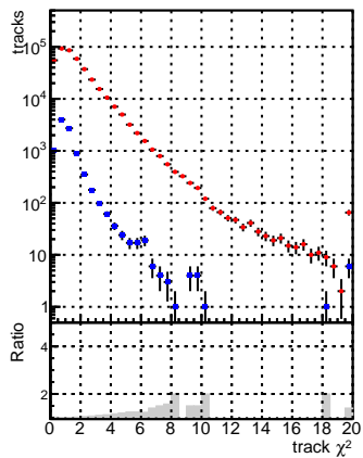
N of reco track vs. DQM V0001 R000000001 Global mkFitbase RECO DQM V0001 R000000001 Global CMSSW X_Y_Z_RECO
