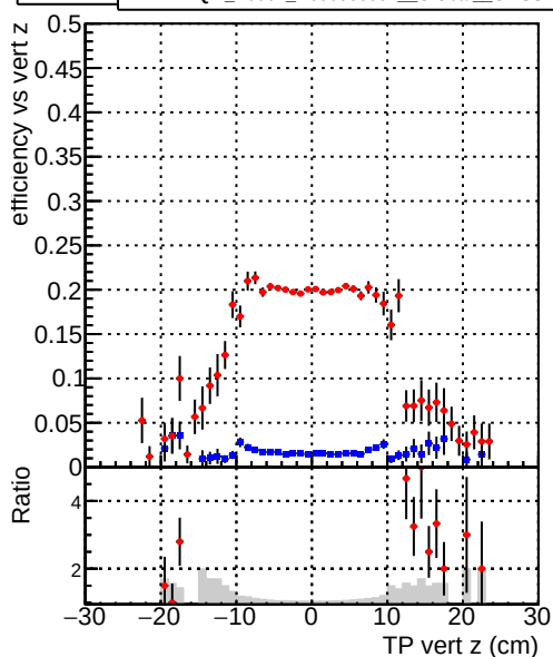
Efficiency vs vert z — DQM_V0001_R0000000001_Global_mkFitbase_RECO — DQM_V0001_R0000000001_Global_CMSSW_X_Y_Z_RECO
