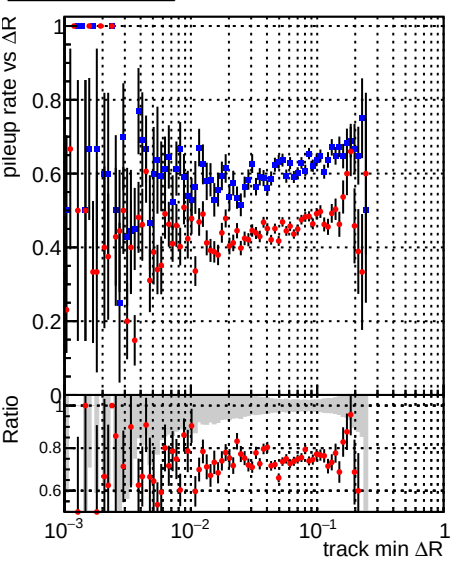
Legend: DQM_V0001_R000000001_Global_mkFitbase_RECO (blue), DQM_V0001_R000000001_Global_CMSSW_X_Y_Z_RECO (red)
