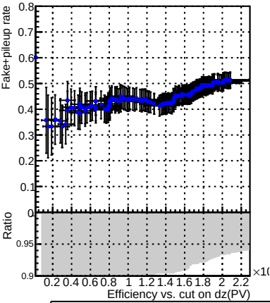
DQM_V0001_R000000001_Global_mkFitbase_RECO
