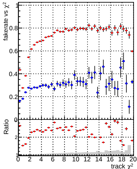
Fake rate vs. DQM_V0001_R0000000001 Global mkFitbase RECO Fake rate vs. Global mkFitbase RECO Duplicates Rate vs. Global mkFitbase RECO Pileup rate vs. Global mkFitbase RECO
