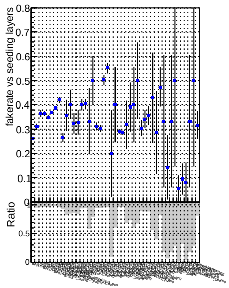
Fake rate vs. DQM V0001_R000000001 Global mkFitbase RECO Fake rate vs. DQM V0001_R000000001 Global CMSSW X Y Z RECO
