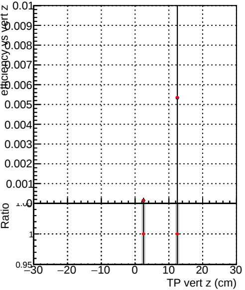
Efficiency vs vertpos Legend: DQM_V0001_R000000001_Global_mkFitbase_RECO DQM_V0001_R000000001_Global_mkFit-cand_RECO
