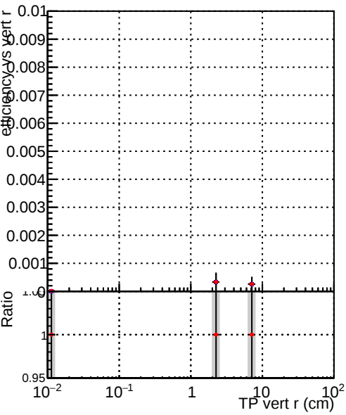
Efficiency vs vertpos Legend: DQM_V0001_R000000001_Global_mkFitbase_RECO DQM_V0001_R000000001_Global_mkFit-cand_RECO
