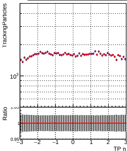
Legend: DQM_V0001_R000000001_Global_mkFitbase_RECO (blue squares), DQM_V0001_R000000001_Global_mkFit-cand_RECO (red circles)
