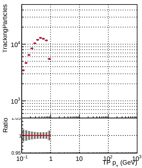
Legend: DQM_V0001_R000000001_Global_mkFitbase_RECO (blue squares), DQM_V0001_R000000001_Global_mkFit-cand_RECO (red circles)
