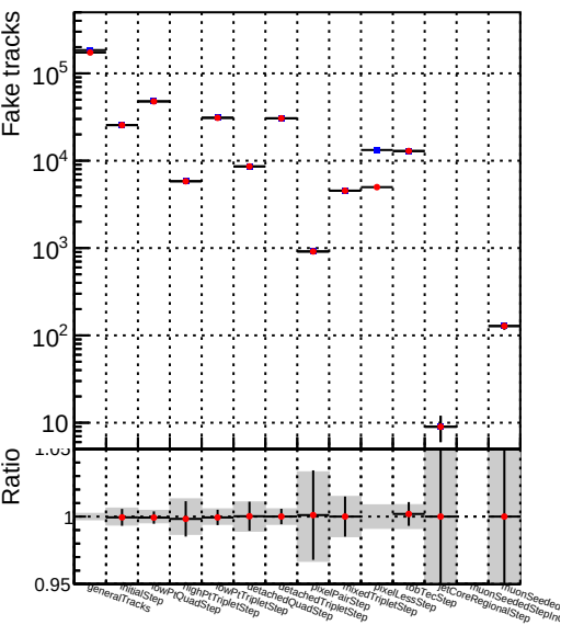
Number ● DQM_V0001_R000000001_Global_mkFit-cand_RECO
