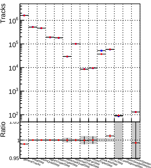
DQM_V0001_R0000000001_Global_mkFitbase_RECO
