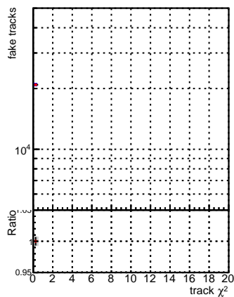
Global_mkFitbase_RECO Global_mkFit-cand_RECO
