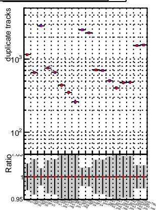
Global_mkFitbase_RECO Global_mkFit-cand_RECO
