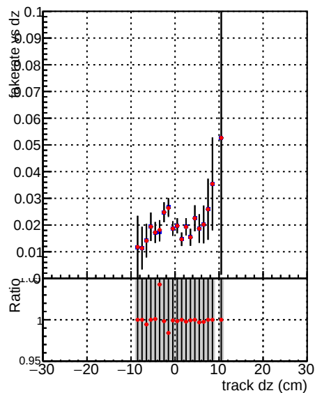
Global mkFitbase RECO Fake rate vs dz █ █ █ Duplicates Rate vs dz █ █ █ Pileup rate vs dz █ █ █
