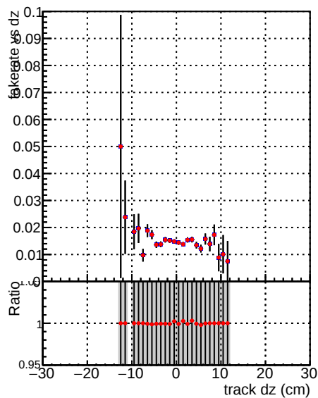
Fake rate vs d DQM V0001_R0000000001_Global_mkFitbase_RECO DQM V0001_R0000000001_Global_mkFit-cand_RECO
