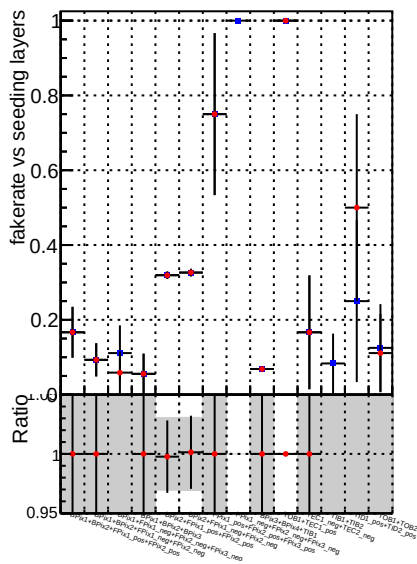
Fake rate vs. DQM V0001_R000000001 Global mkFitbase RECO Fake rate vs. Duplicates Rate vs. Pileup rate vs.
