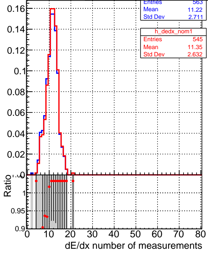
■ DQM_V0001_R000000001_Global_mkFitbase_RECO ● DQM_V0001_R000000001_Global_mkFit-cand_RECO
