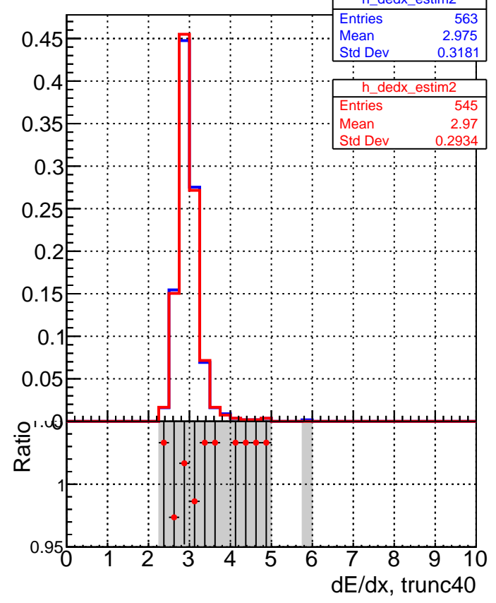
■ DQM_V0001_R000000001_Global_mkFitbase_RECO ● DQM_V0001_R000000001_Global_mkFit-cand_RECO
