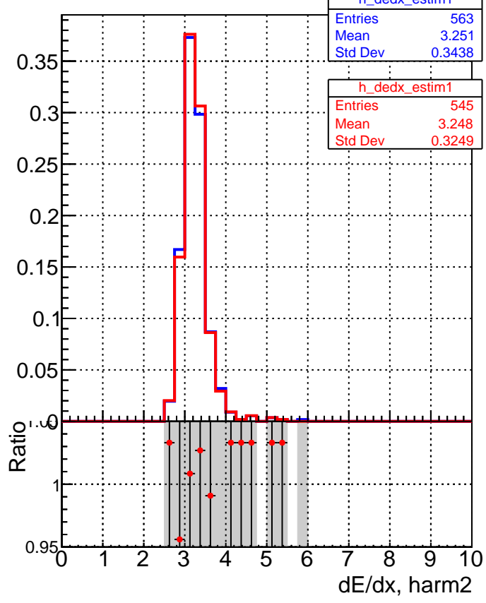
■ DQM_V0001_R000000001_Global_mkFitbase_RECO ● DQM_V0001_R000000001_Global_mkFit-cand_RECO
