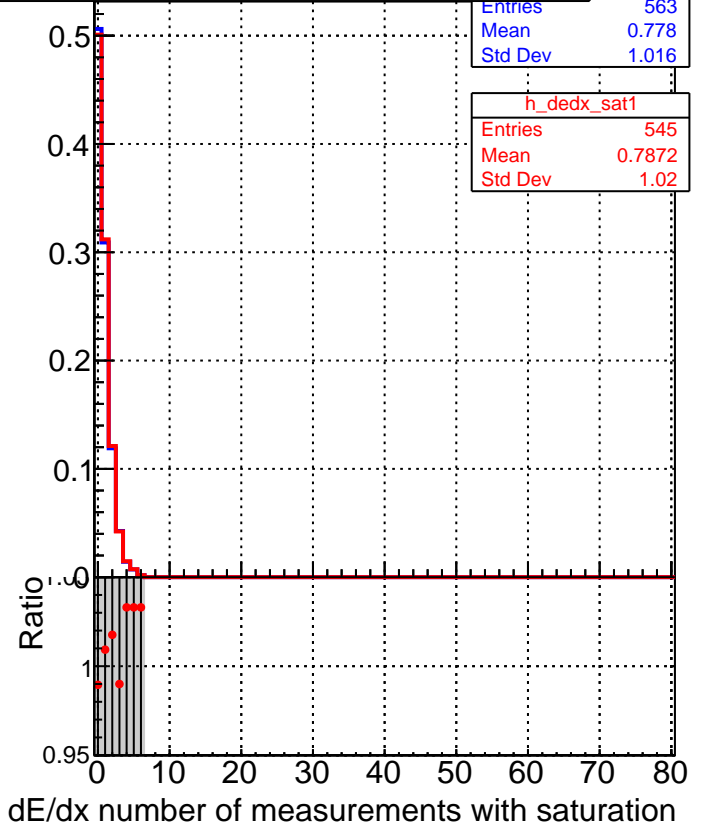
■ DQM_V0001_R000000001_Global_mkFitbase_RECO ● DQM_V0001_R000000001_Global_mkFit-cand_RECO
