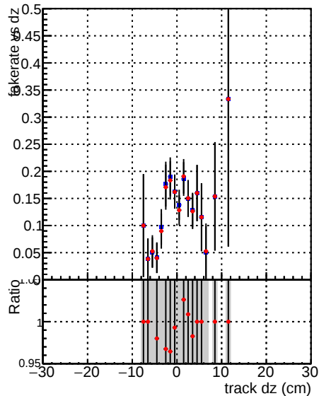
Fake rate vs d DQM V0001_R0000000001_Global_mkFitbase_RECO DQM V0001_R0000000001_Global_mkFit-cand_RECO
