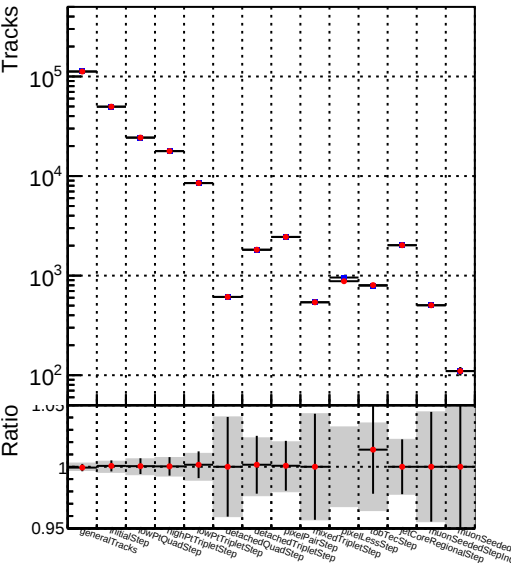
DQM_V0001_R0000000001_Global_mkFitbase_RECO
