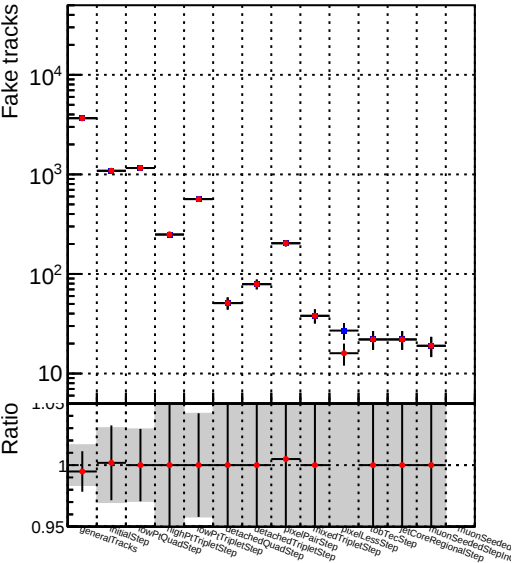
Numbe —●— DQM_V0001_R000000001_Global_mkFit-cand_RECO
