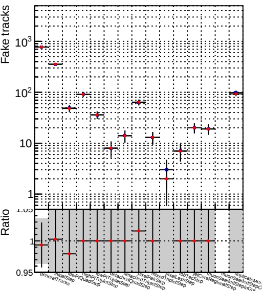
Number —●— DOM V0001 R0000000001 Global mkFit-cand RECO
