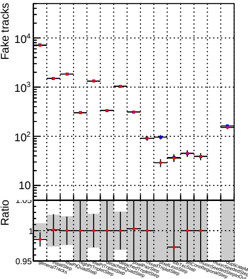
Number —● DQM_V0001_R0000000001_Global_mkFit-cand_RECO
